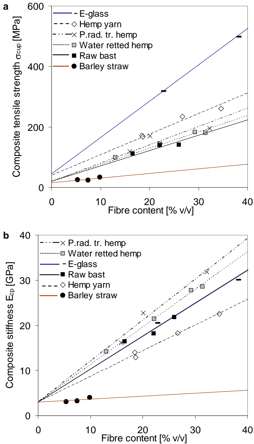
Figure 38. Tensile strength and stiffness for the composites corrected for porosity versus fibre content (Paper IV+unpublished data).
