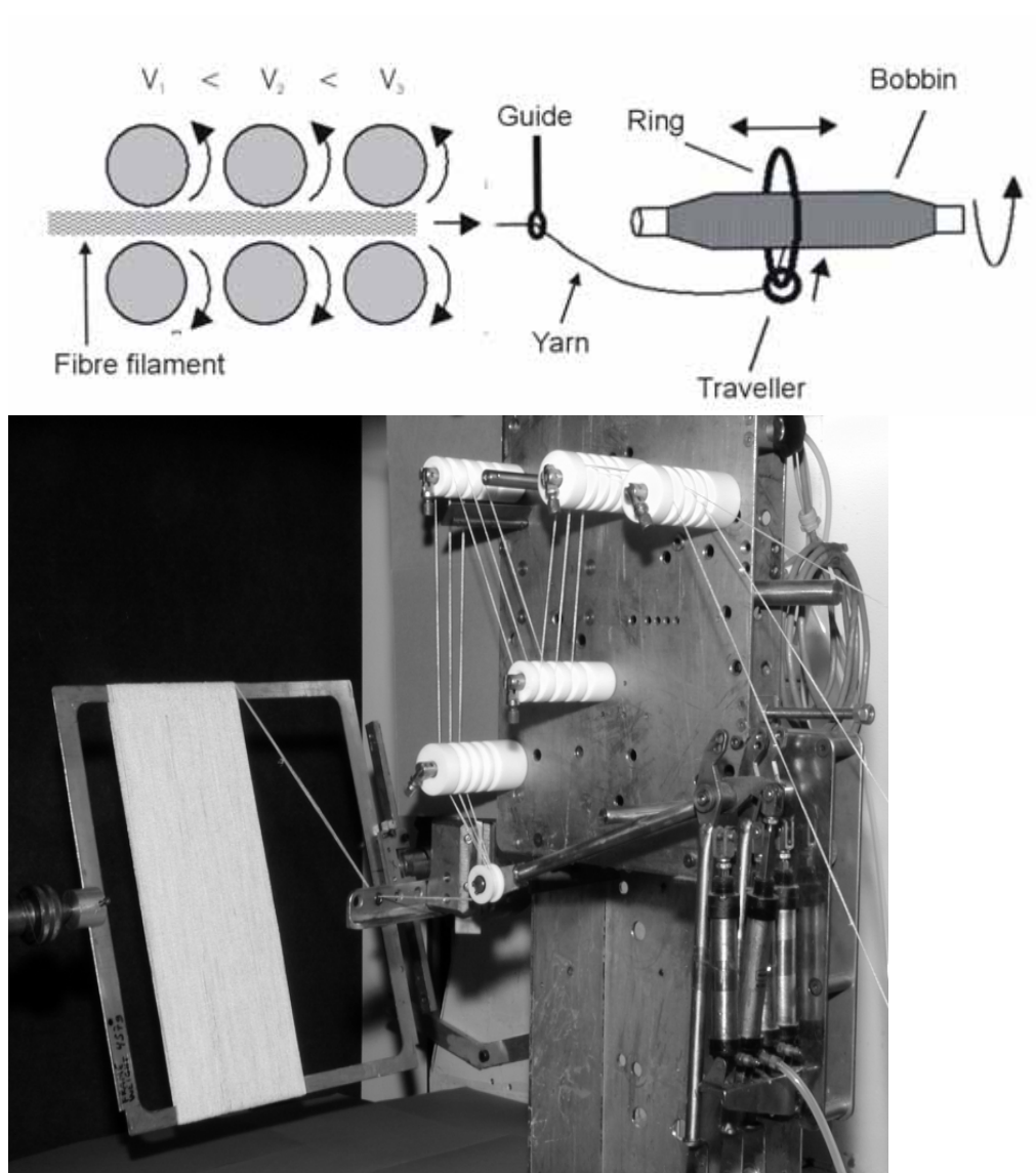
Figure 18. From fibre filament to aligned fibre assemblies: The drafting process with three pairs of rollers at different rotation speed ( v ; left), followed by ring spinning to get yarn (Grosberg and Iype, 1999; centre) and filament winding of yarn to get aligned fibre assemblies (Modified from Madsen, 2004; right).
