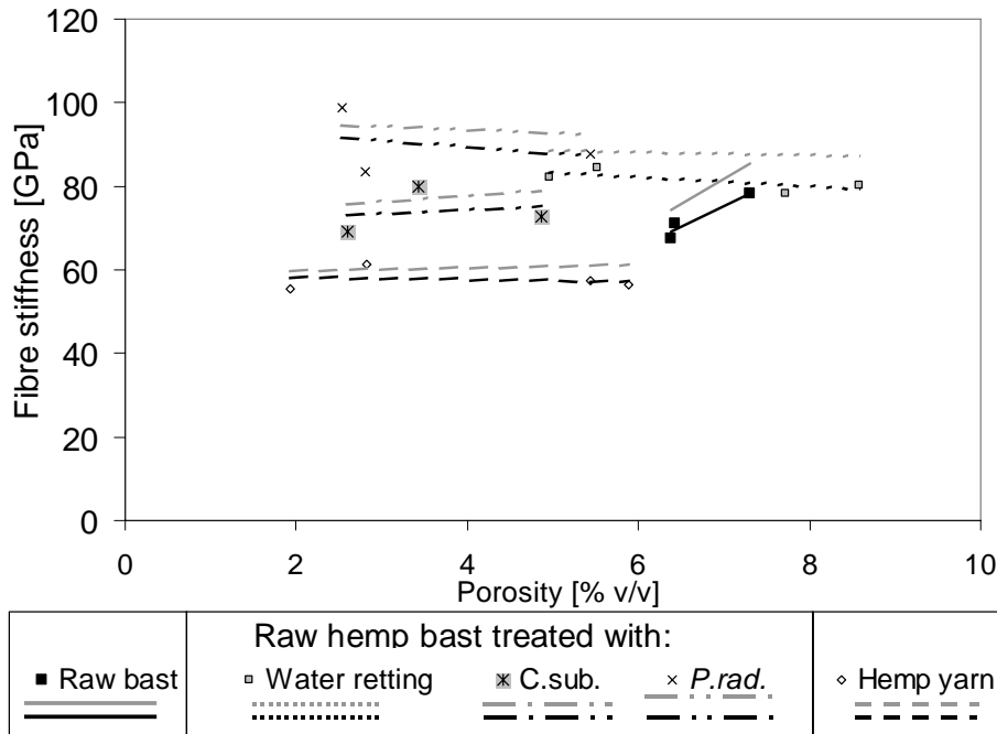
Figure 36. Tensile strength (a) and stiffness (b) calculated for the fibres versus composite porosity with n_\sigma = 2.1 and n_E=1 . The markers and black regression lines represent results not corrected for porosity and the grey regression lines represent the results with correction of the composite properties for porosity (unpublished data).
