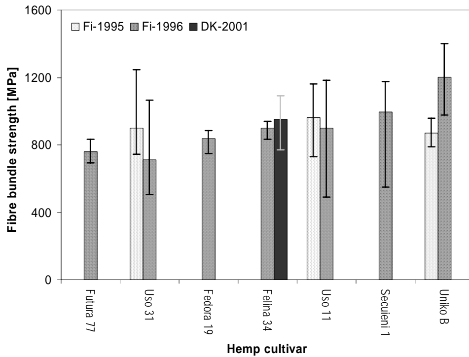
Figure 28. Fibre bundle strength of fibres from the hemp cultivars grown by Sankari (2000) in Finland. For the Finish samples, the test span length was 20 mm. For the fibres from Felina 34 that was grown at Danish Institute of Agricultural Sciences in 2001(DK-sample), the test span length was 3 mm. The cultivars are sorted according to increasing average strength.
