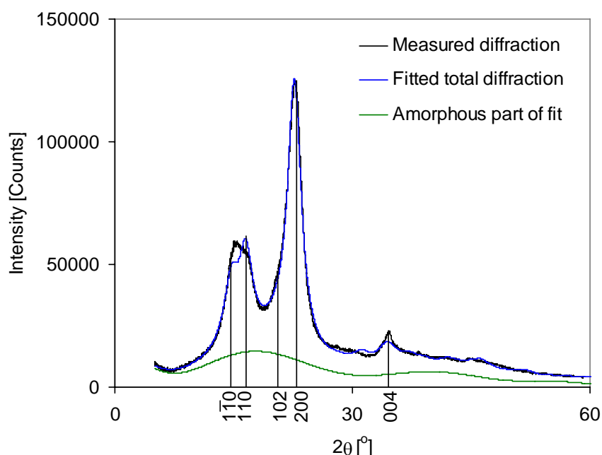
Figure 13. Diffraction pattern of water retted hemp fibres measured in reflection mode of a side-loaded fibre sample. Determination of the crystalline cellulose content was done by Rietveld refinement. The obtained fits for the amorphous and the crystalline diffraction are shown (further details in Paper III). The peak positions are marked with Miller indices.
