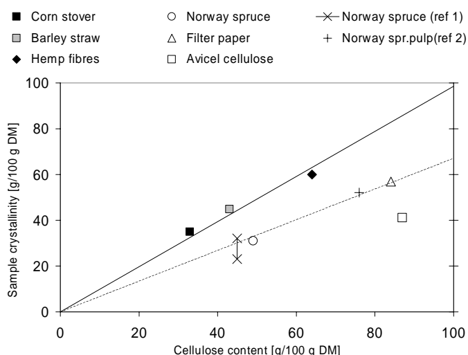
Figure 14. Sample crystallinity determined by Rietveld refinement compared to the cellulose content. The relationship for non-woody materials (full drawn line) and the relationship for wood based materials (dotted line) are shown (ref 1 = Andersson et al. (2003); ref 2 = Liitia et al., (2003); Paper III; Paper IV).
