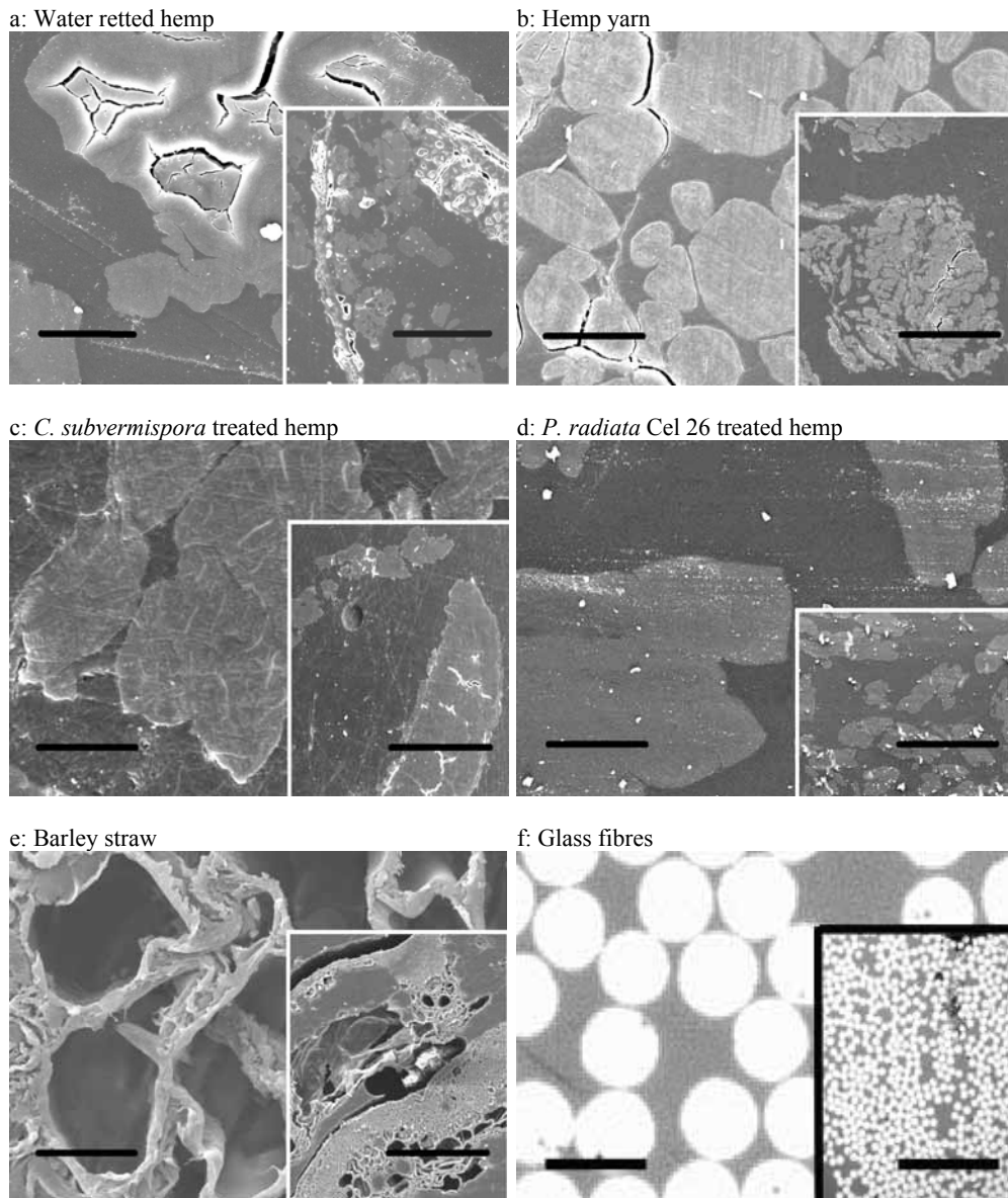
Figure 33. SEM microscopy photos of transverse composite sections recorded at low and high magnification with the applied fibres. The small inset pictures have a scale bar length of 200 µm and the background pictures 20 µm (Paper IV; unpublished data).
