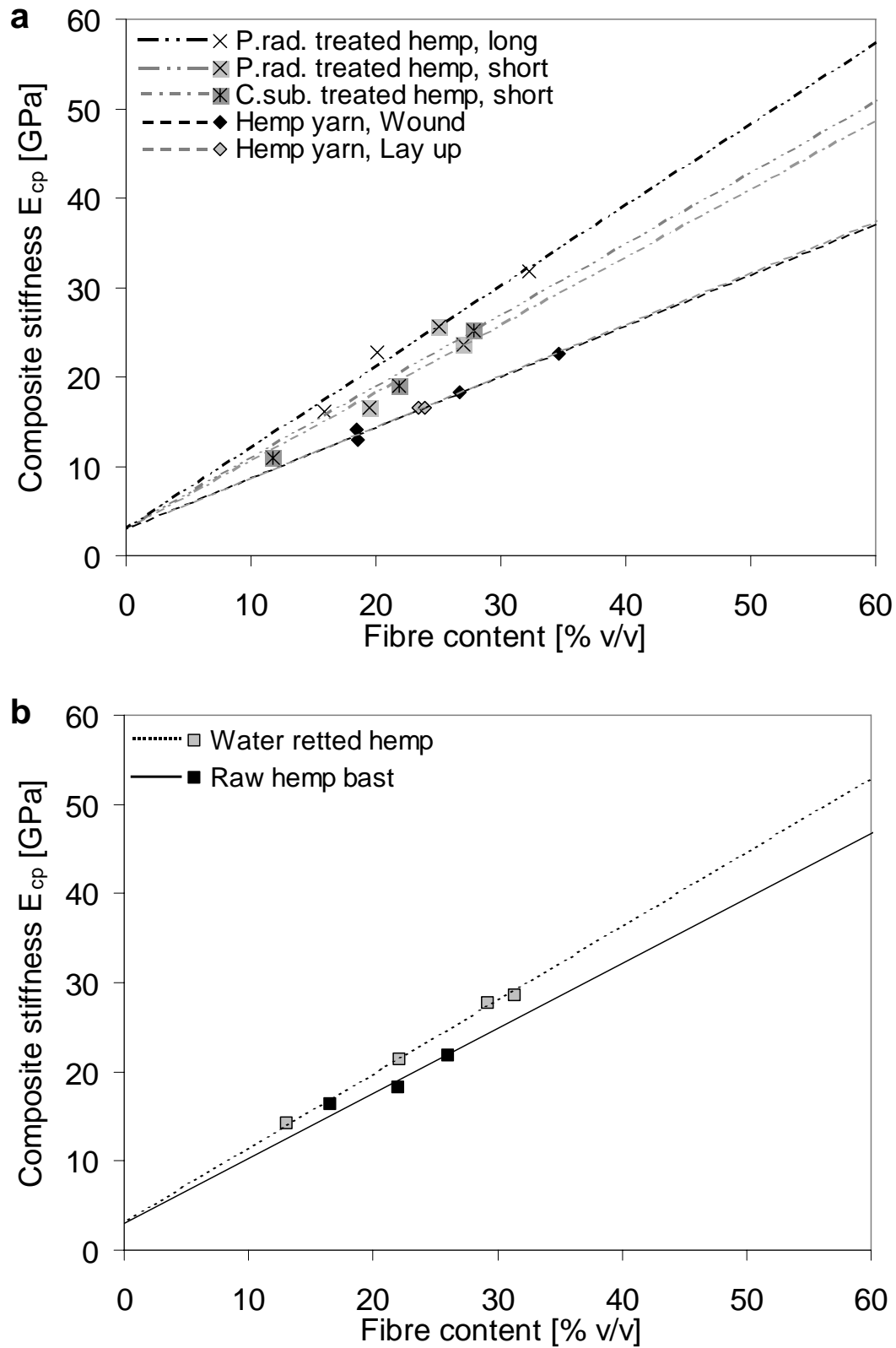
Figure 7. Effect of composite fabrication (a), fibre length (a), fungal defibration (a) and water retting (b) on composite stiffness after correction for porosity plotted as a function of fibre volume fraction.
